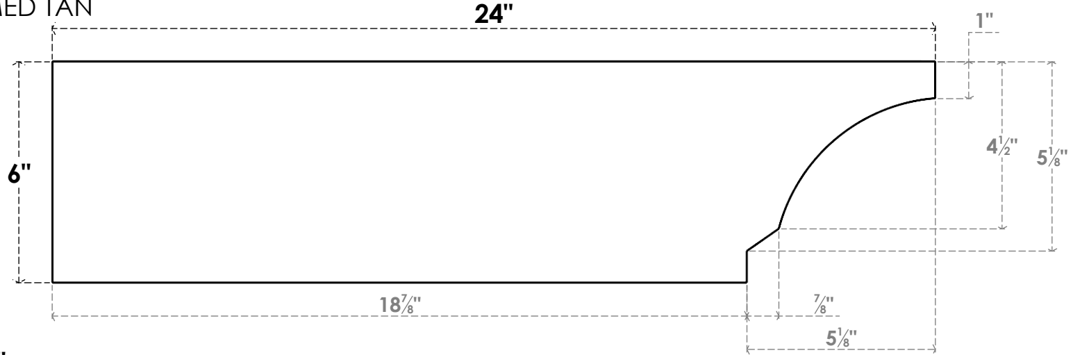
SIDE PROFILE
